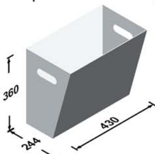
M0101 Waste Bin
